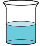
1 mol \text{MgCl}_2
